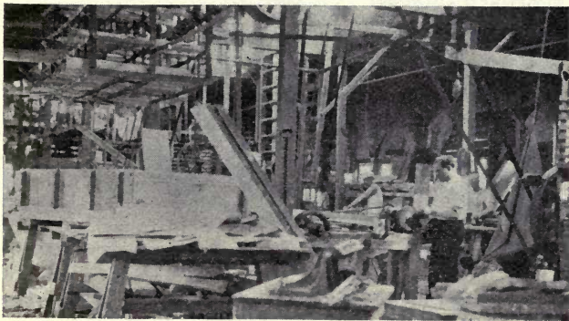
FIG. 33—GENERAL VIEW OF WOOD PATTERN SHOP IN FACTORY MAKING ORNAMENTAL AND TRIM STONE EXCLUSIVELY
